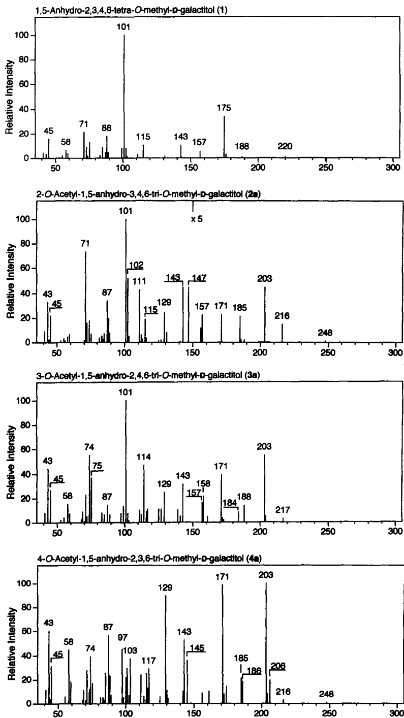
Fig. 1. Electron-ionization mass spectra of the methylated 1,5-anhydro-D-galactitol acetates (compounds 1 and 2a–16a).
